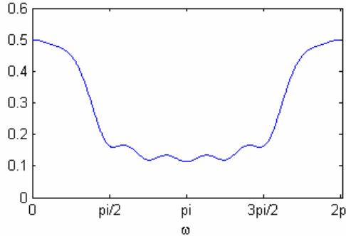
Magnitude responses
