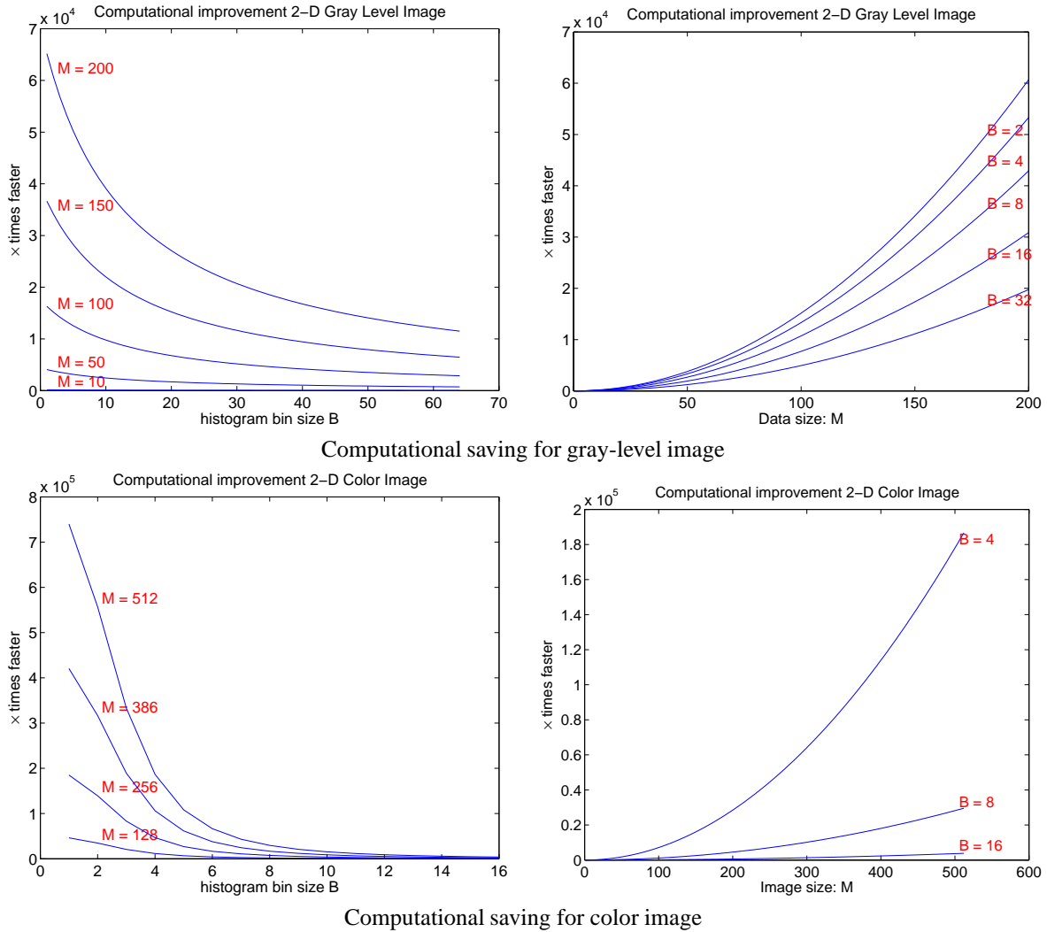
Figure 2. Achieved computational reduction in comparison to conventional method. The integral histogram method is as many times as faster than the existing approach.
