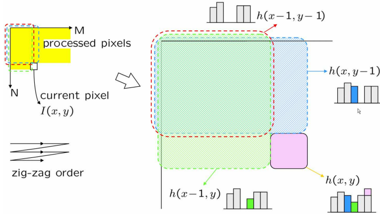
Figure 1. Propagation of integral histogram. Yellow indicates already traversed points. At each recursion along the zig-zag order, the current integral histogram is obtained from the integral histogram values of the three neighbors, and the bin that corresponds to current points value is increased by one.
