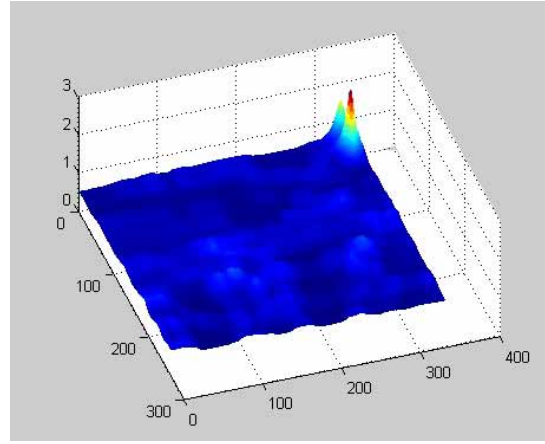
similarity
