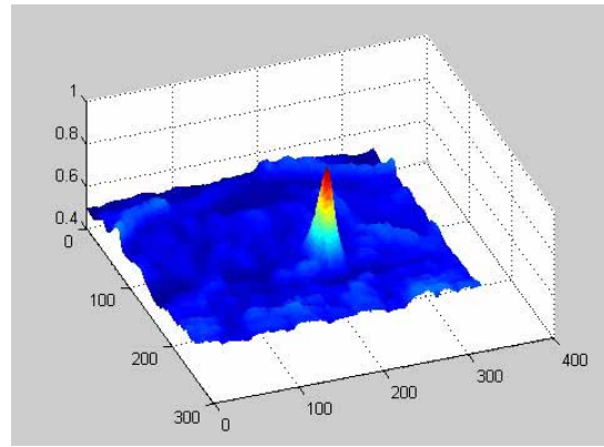
similarity
